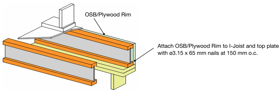
Diagram 1C Rim I-Joist at Exterior Wall
