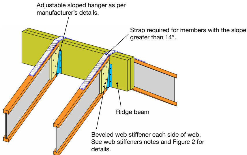
Diagram 2A Ridge Beam Rafter Connection
