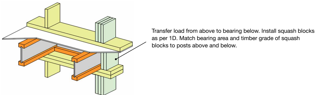
Diagram 1F Double I-Joist Rim
