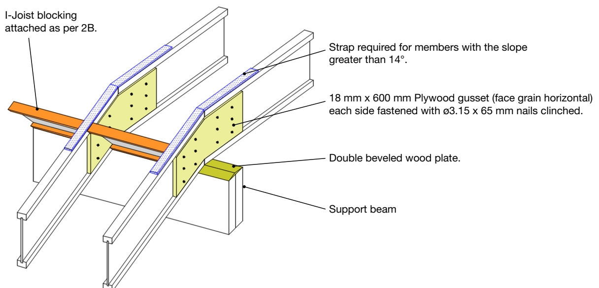
Diagram 2C Rafter Connection with Fitted Plywood Gusset
