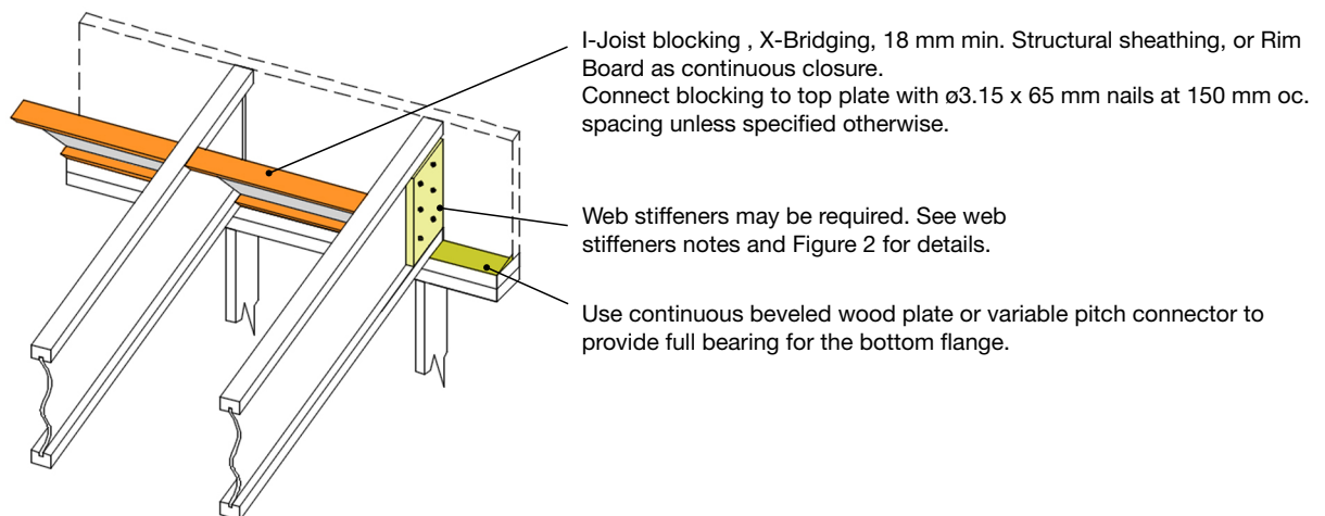
Diagram 2B Upper End, Rafters Bearing on Wall
