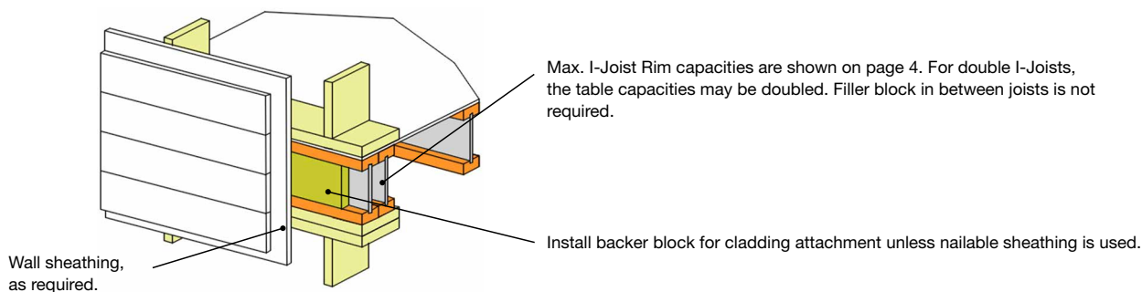
Diagram 1F Double I-Joist Rim
