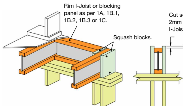
Diagram 1D Squash Blocks
