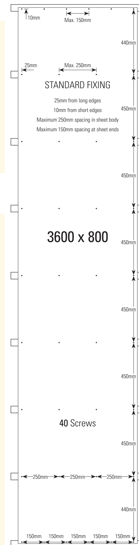
Figure 3. Fixing plan
