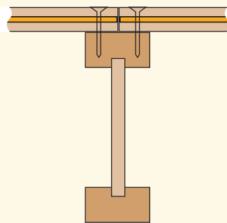
Figure 4. Fixing to EWP I-Beam
